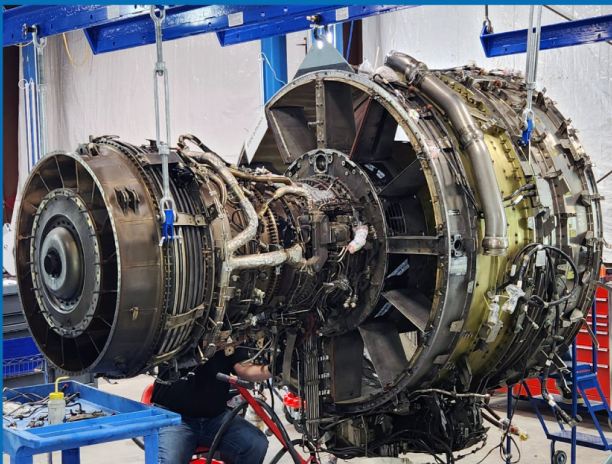
CFM56-5B/7B engine at Jet AirWerks' Engine Services Centre
